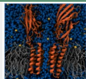
MD simulations /GROMACS/
