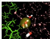
QM/MM /CPMD/
