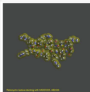
Docking /HADDOCK/
